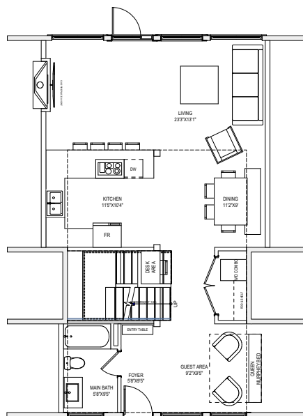
MAIN FLOOR
