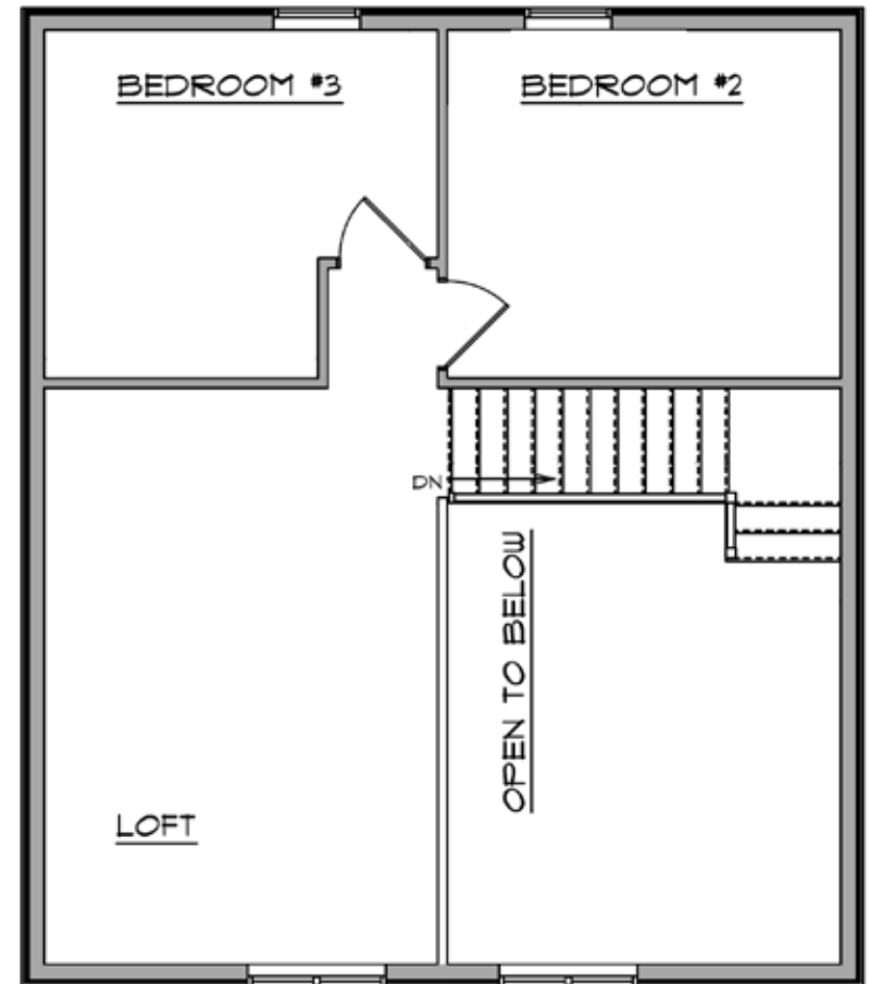
UPPER FLOOR
