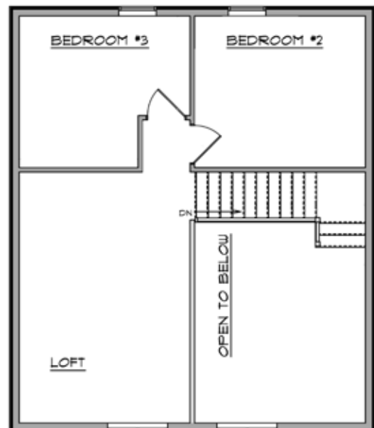
UPPER FLOOR
