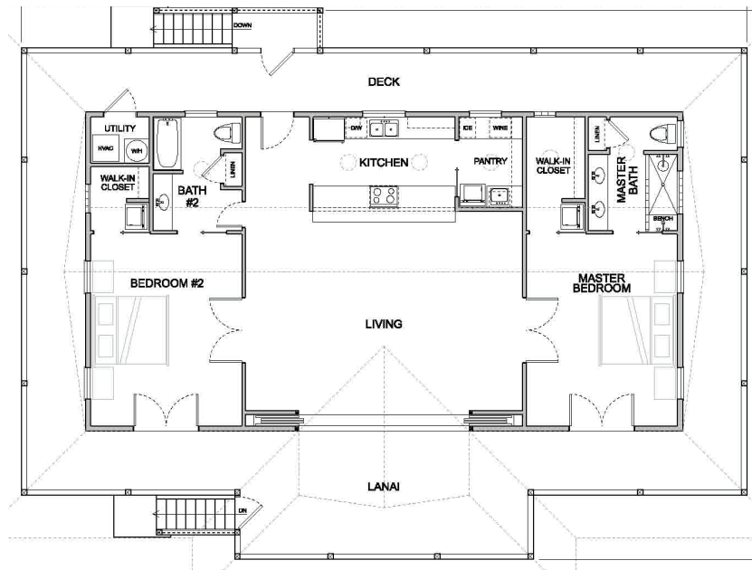
MAIN FLOOR
