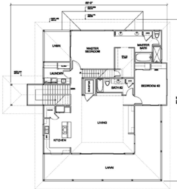
SECOND FLOOR
