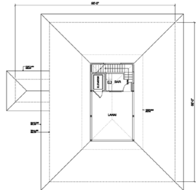
THIRD FLOOR
