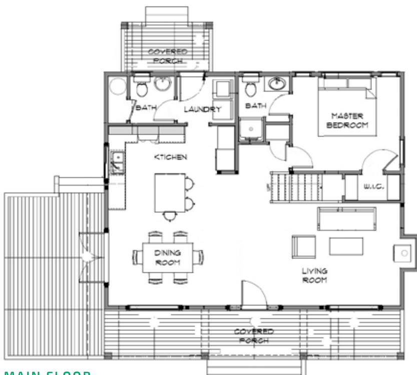
MAIN FLOOR
