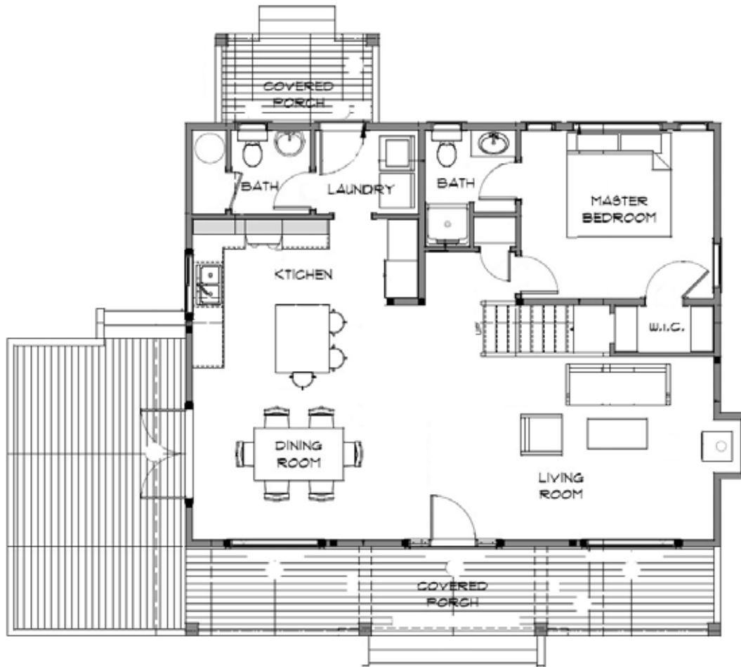
MAIN FLOOR
