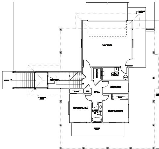
LOWER FLOOR
